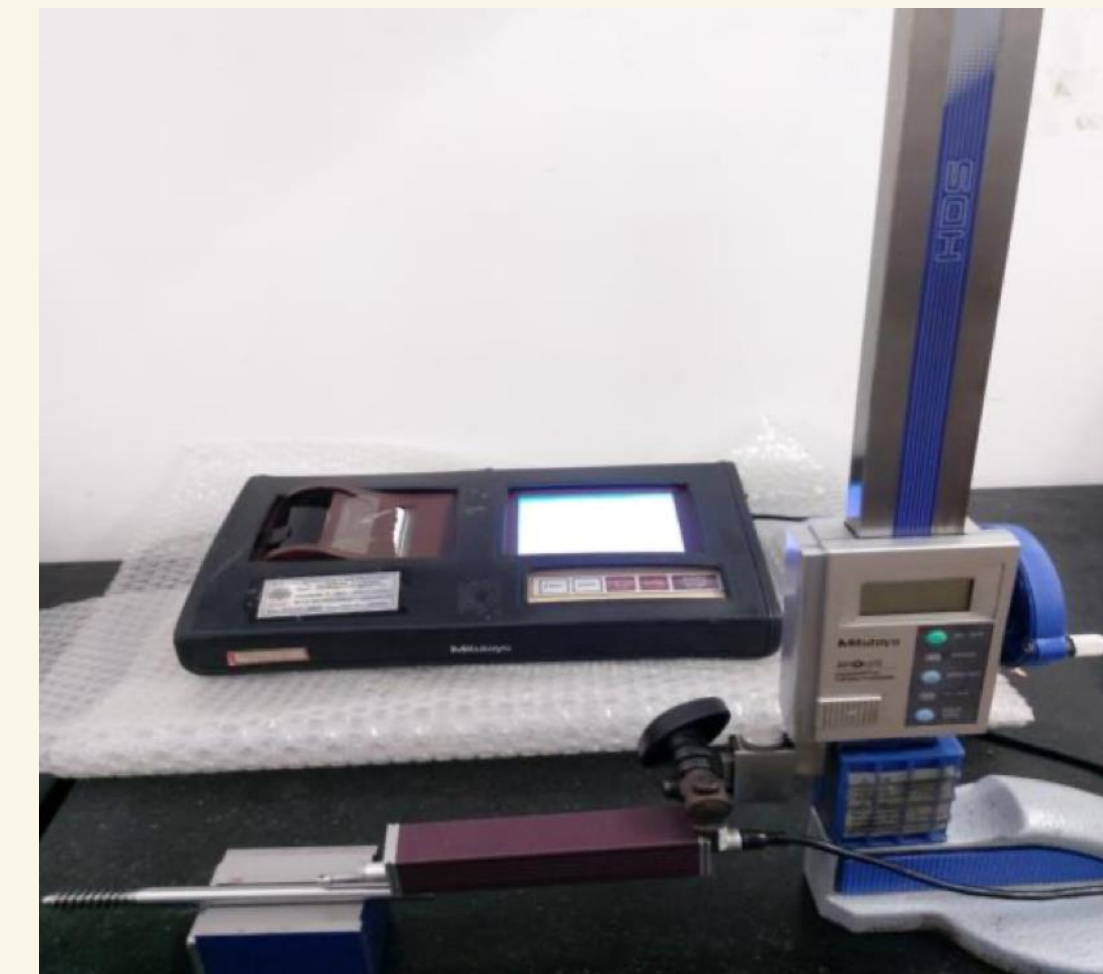
ROUGHNESS TESTER
